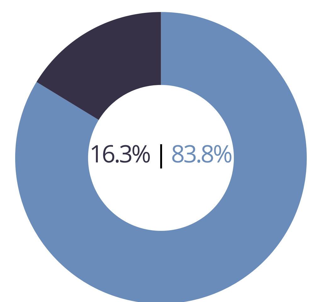
Quartile 4 (upper)
